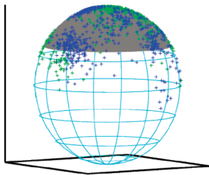
Figure 2. Distribution of orientations of bond 17 of NPG extracted from the REMD simulation of the P450 BM-3/NPG corresponding to the proximal (blue) and distal (green) states oriented, with the mean orientation pointing along an orientation perpendicular to the plane. The gray shaded area represents the distribution resulting from diffusion in a cone which best represents the distribution of orientations (same S^2 and mean orientation) from the simulation.
